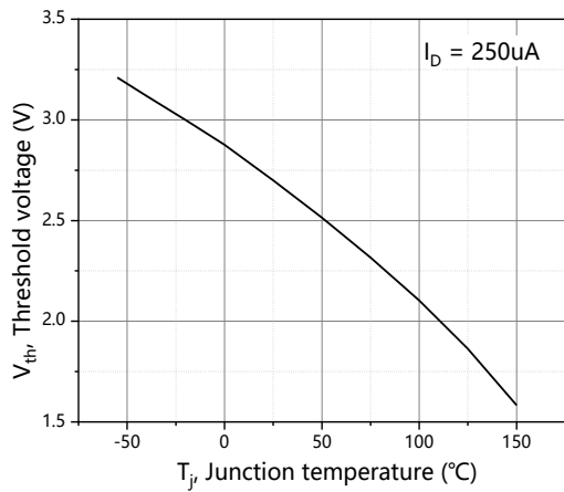
Figure 7. Threshold voltage
