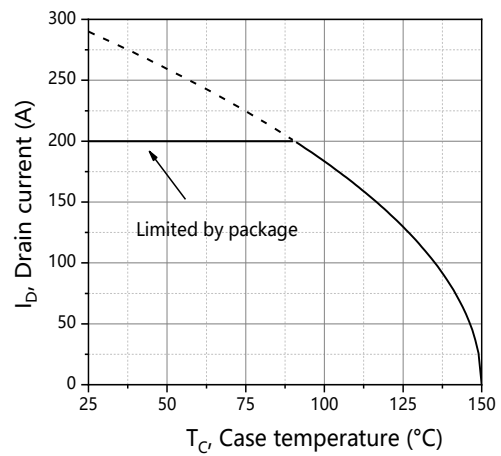
Figure 10. Drain current
