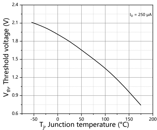
Figure 7. Threshold voltage
