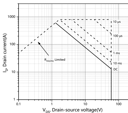
Figure 11. Safe operation area T_C=25^{\circ}\text{C}
