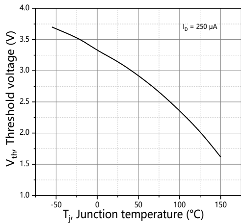
Figure 7. Threshold voltage
