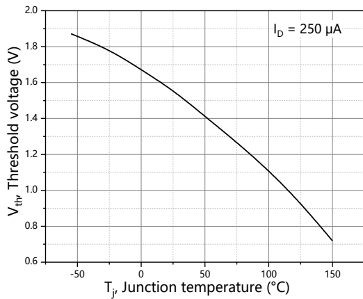
Figure 7. Threshold voltage
