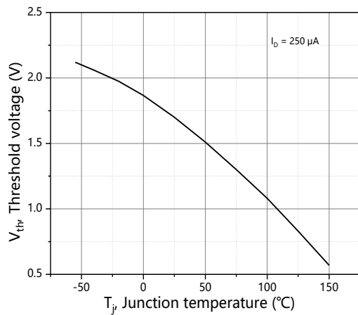
Figure 7. Threshold voltage
