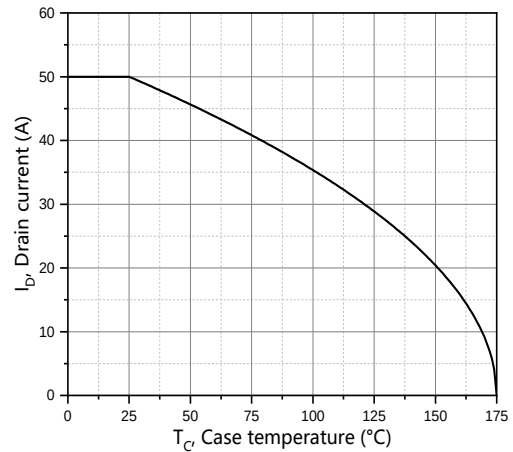
Figure 10. Drain current
