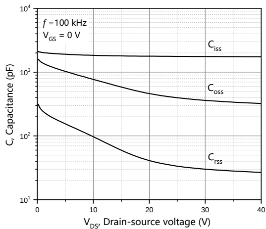
Figure 3. Typ. capacitances
