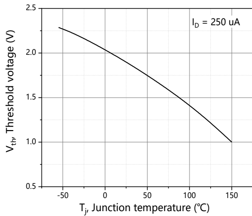
Figure 7. Threshold voltage
