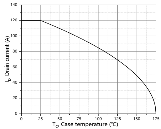
Figure 10. Drain current
