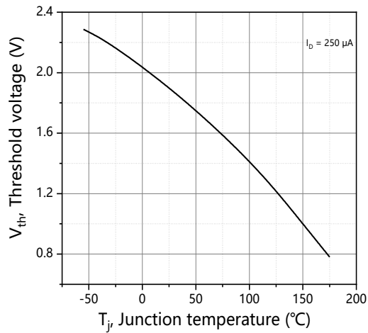
Figure 7. Threshold voltage
