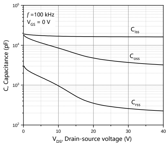
Figure 3. Typ. capacitances
