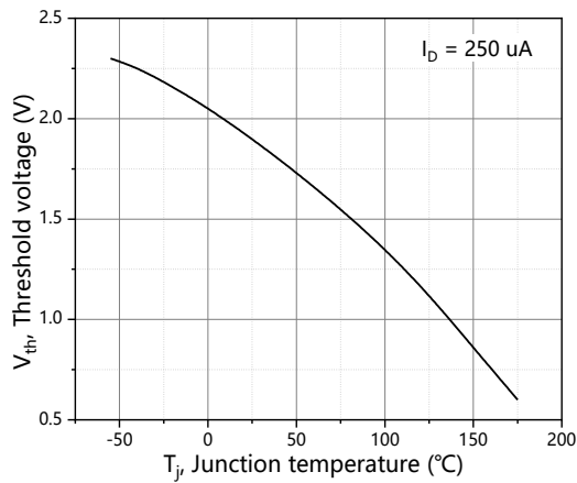
Figure 7. Threshold voltage
