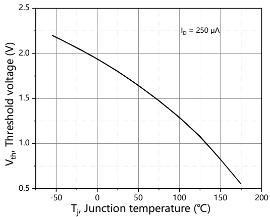
Figure 7. Threshold voltage
