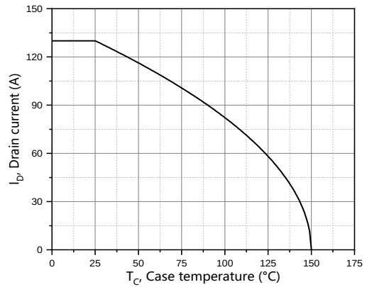
Figure 10. Drain current
