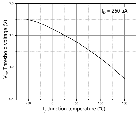
Figure 7. Threshold voltage
