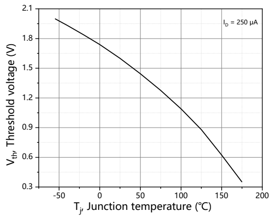
Figure 7. Threshold voltage
