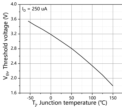
Figure 7. Threshold voltage
