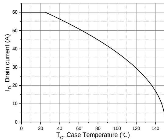
Figure 8. Drain current
