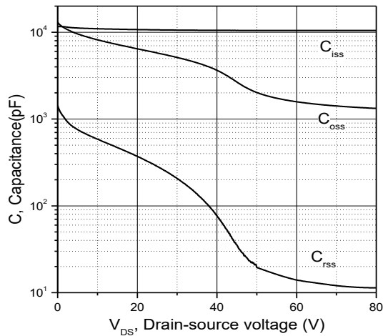
Figure 3. Typ. capacitances
