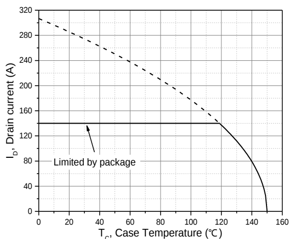
Figure 8. Drain current
