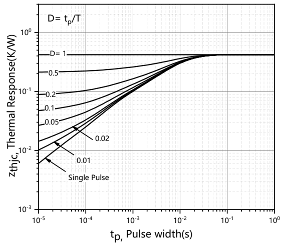
Figure 10. Max. transient thermal impedance
