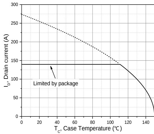
Figure 8. Drain current
