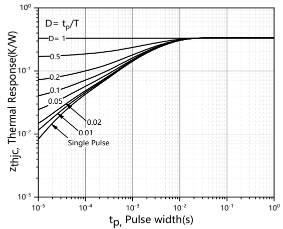
Figure 10. Max. transient thermal impedance
