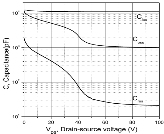
Figure 3. Typ. capacitances
