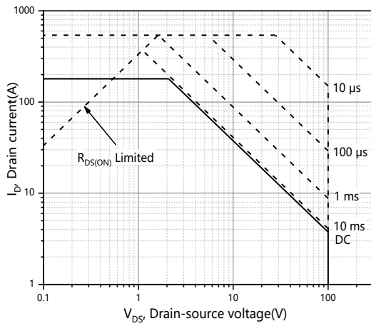
Figure 9. Safe operation area T_C=25\text{ }^{\circ}\text{C}
