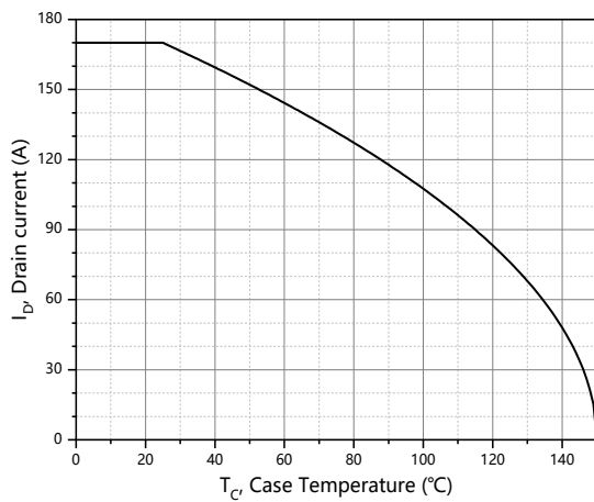
Figure 9. Drain current
