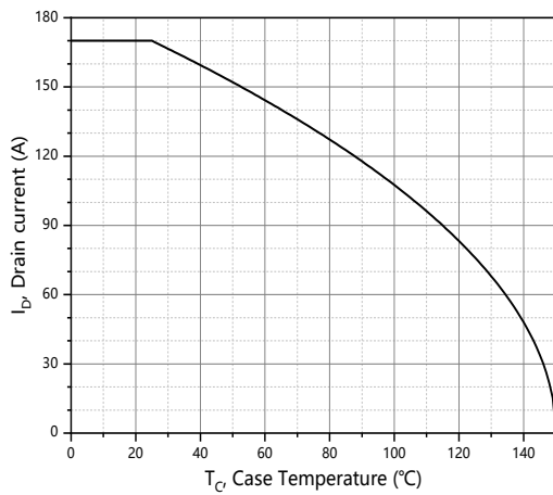
Figure 9. Drain current
