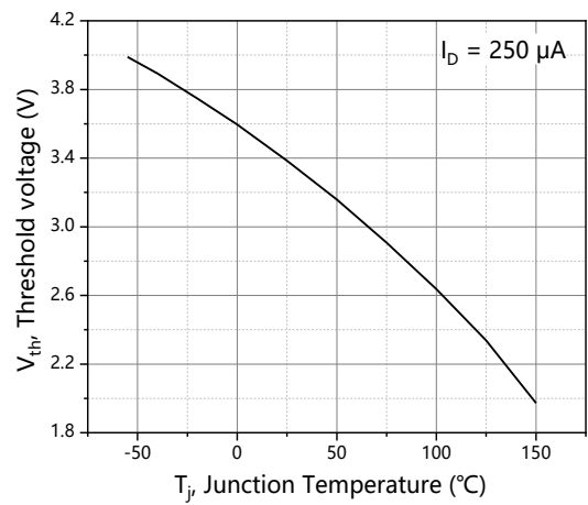
Figure 8. Threshold voltage
