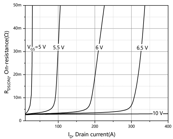
Figure 10. Drain-source on-state resistance
