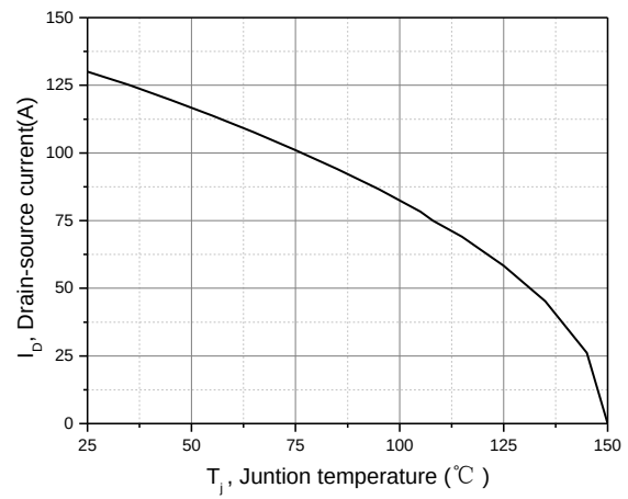
Figure 8. Drain current
