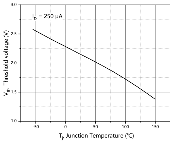
Figure 7. Threshold voltage
