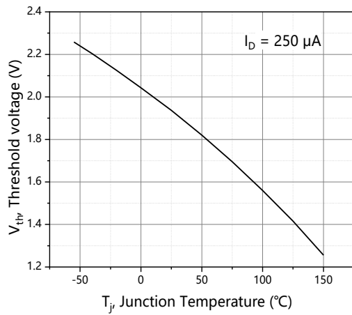
Figure 7. Threshold voltage
