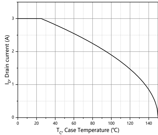
Figure 10. Drain current
