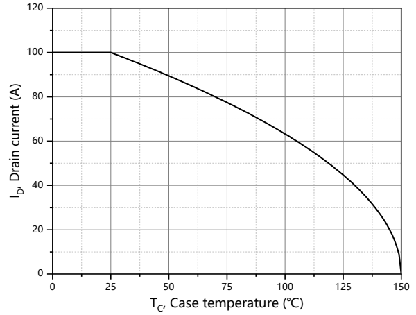
Figure 10. Drain current
