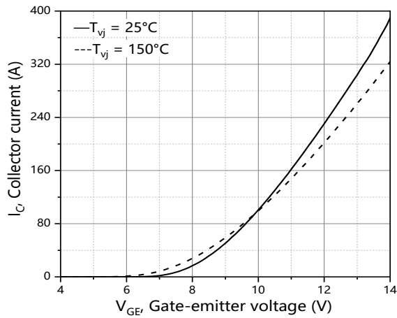
Figure 3. Typical transfer characteristics ( V_{CE}=20\text{ V} )
