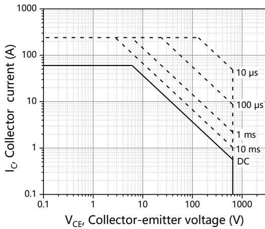
Figure 9. Safe operation area T_C=25^{\circ}\text{C}
