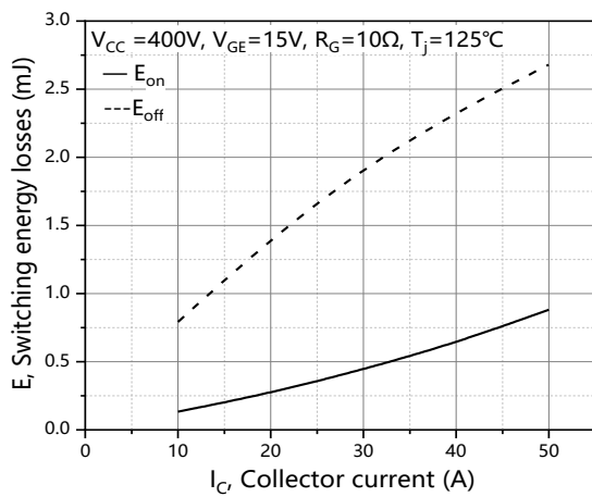
Figure 9. Switching energy vs. collector current
