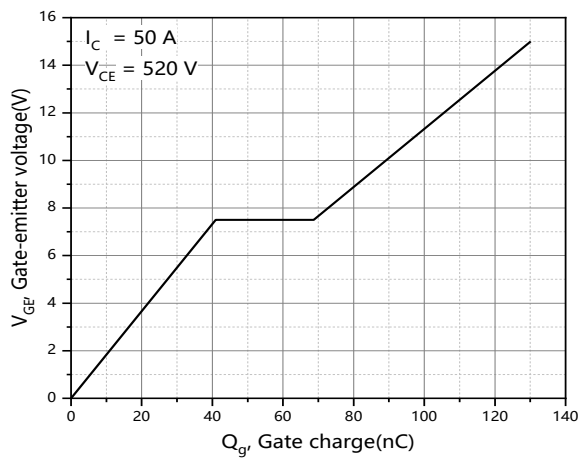
Figure 5. Typical gate charge
