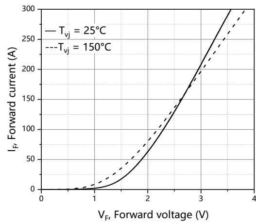
Figure 8. Forward characteristic of diode
