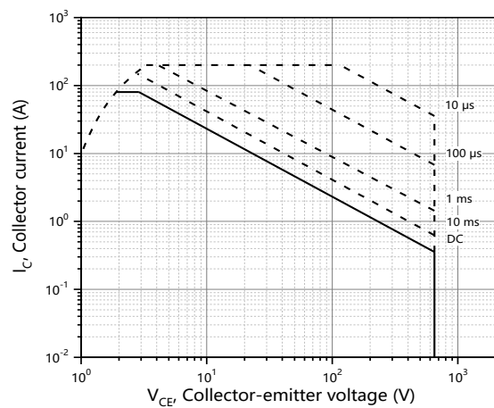
Figure 12. Safe operating area (T_{vj}=25^{\circ}\text{C})
