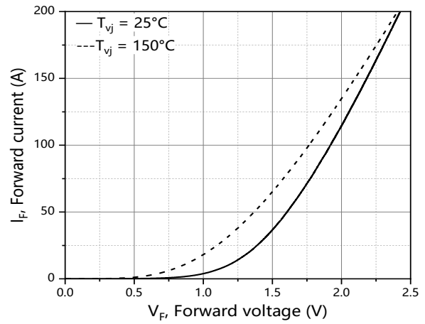
Figure 8. Forward characteristic of diode
