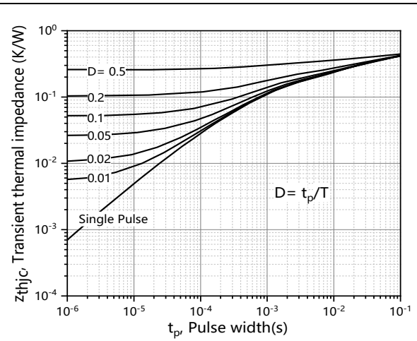
Figure 8. IGBT transient thermal impedance
