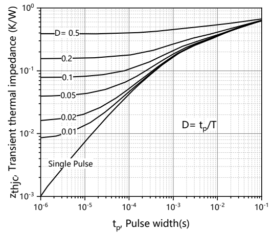
Figure 10. Diode transient thermal impedance
