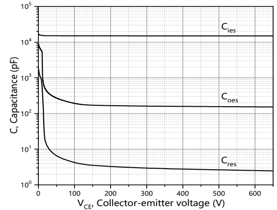
Figure 4. Typical capacitance ( V_{GE}=0\text{V} , f=100\text{ kHz} )
