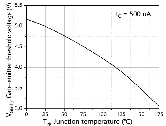
Figure 6. Gate-emitter threshold voltage
