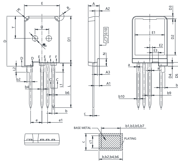
SECTION C-C, D-D & E-E&F-F
