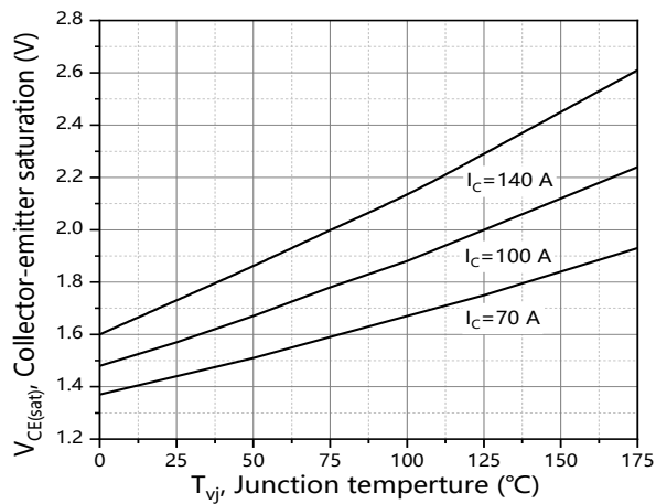
Figure 7. Typical collector-emitter voltage
