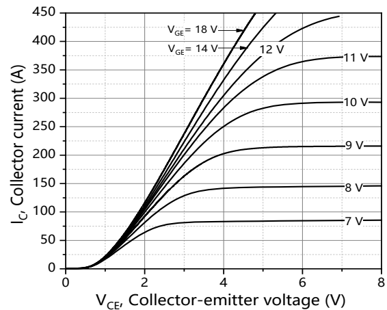
Figure 2. Typical output characteristics ( T_{vj}=150^{\circ}\text{C} )
