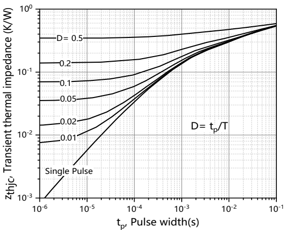
Figure 11. Diode transient thermal impedance
