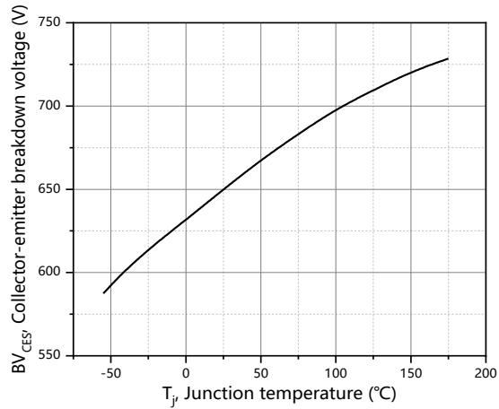
Figure 9. Collector-emitter breakdown voltage
