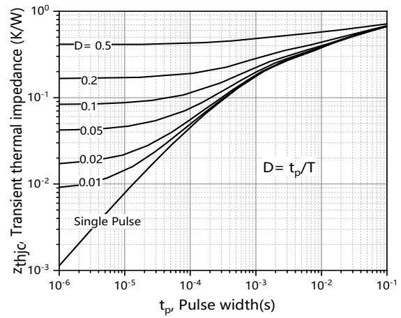
Figure 10. IGBT transient thermal impedance
