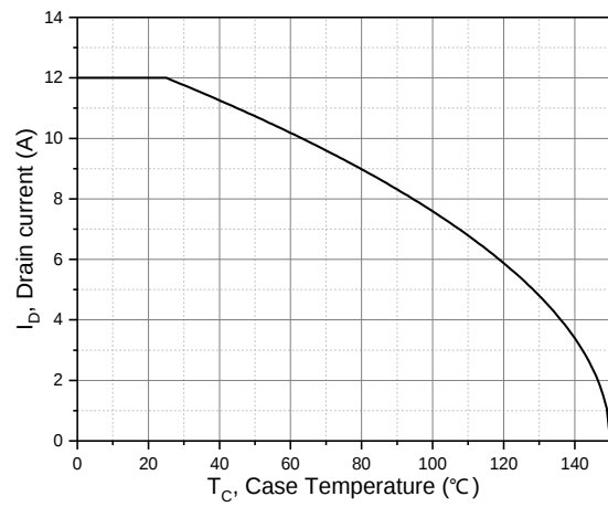
Figure 10. Drain current
