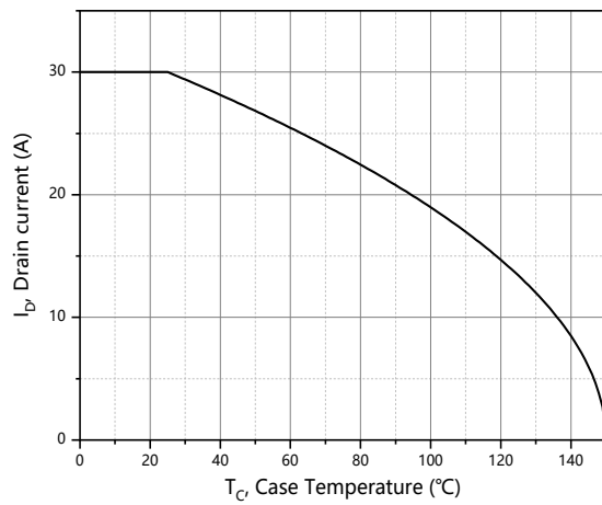
Figure 9. Drain current
