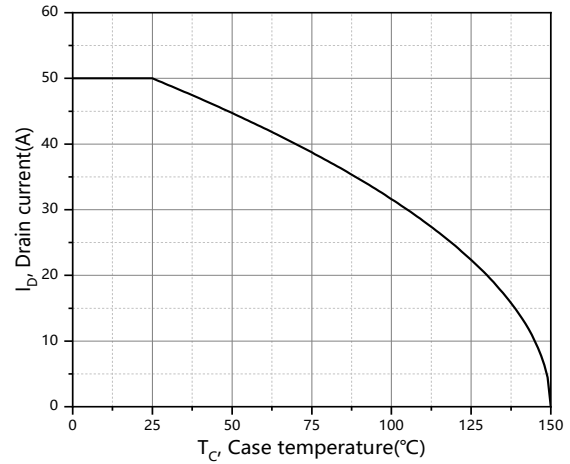
Figure 10. Drain current
