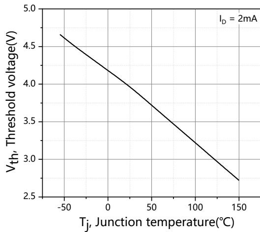
Figure 7. Threshold voltage
