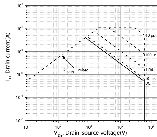
Figure 12. Safe operation area T_c=25^\circ C
