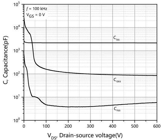
Figure 3. Typ. capacitances
