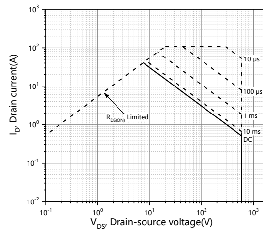
Figure 12. Safe operation area T_c=25^\circ\text{C}
