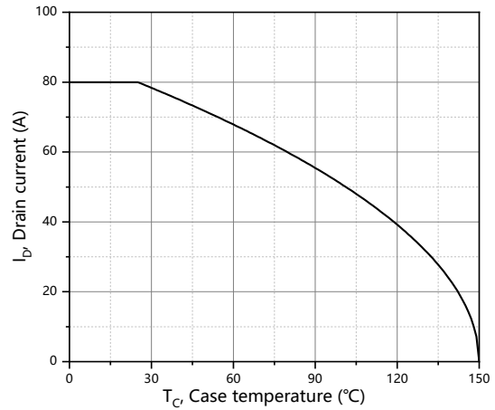
Figure 10. Drain current
