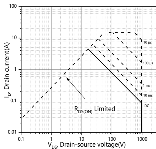
Figure 12. Safe operation area T C =25 °C
